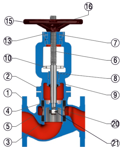
CLASS 300 - DN65 TO 150
