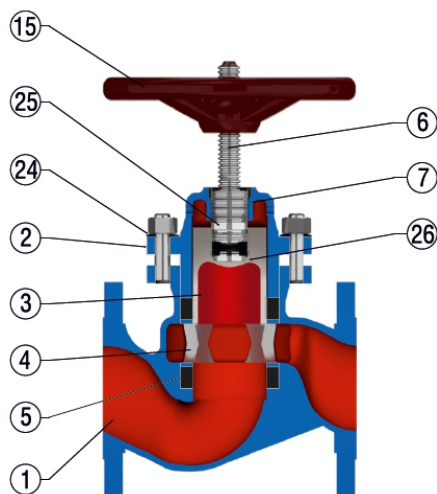
CLASS 150 - DN15 TO 150
